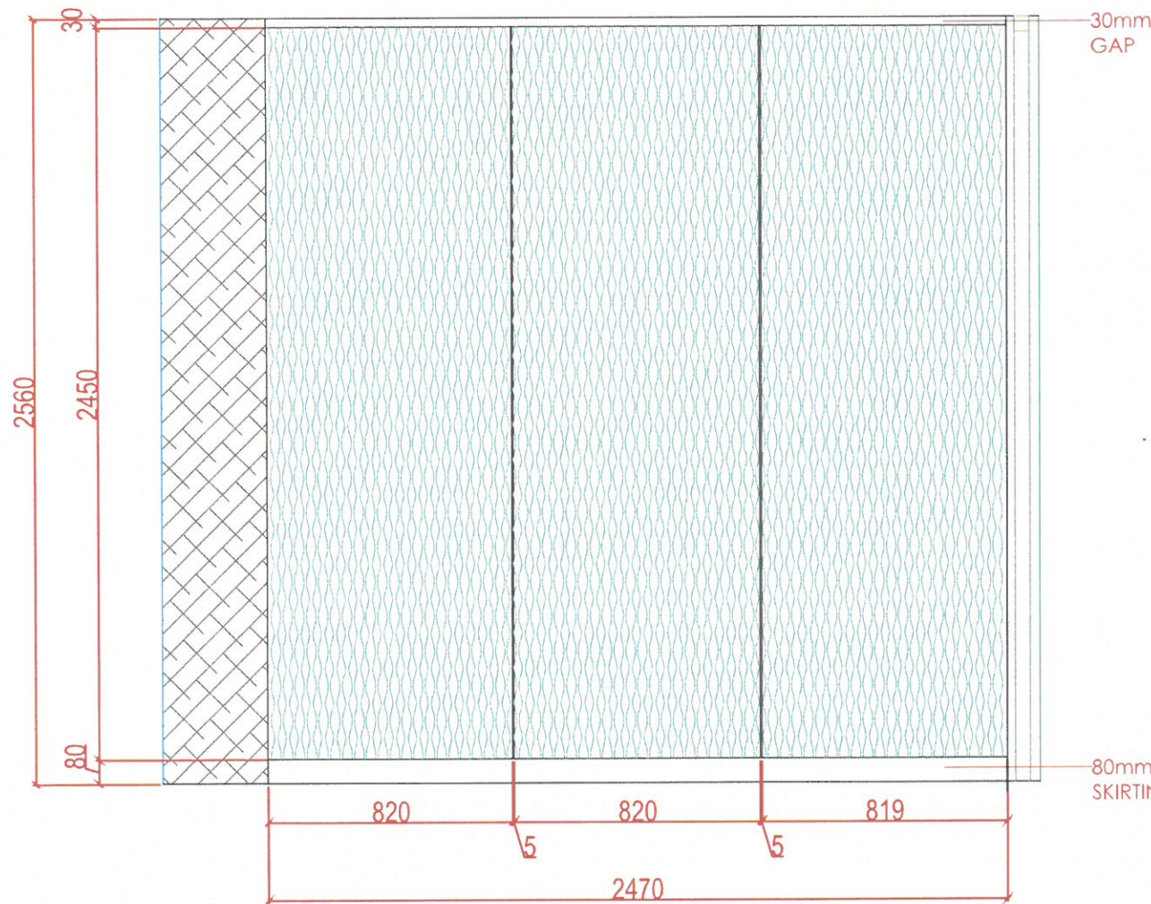
Elevation-A Details
